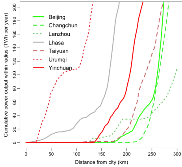
Figures A12 and A13: Proximity of select cities to CSP potential in China (left) and India (right) under Scenario 3
