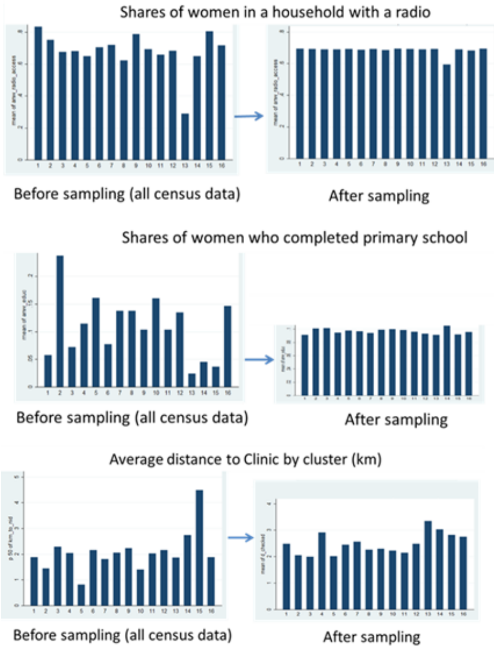
Figure III: Smoothing strategy
